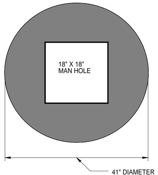
TOP VIEW OF LID WITH MANHOLE
