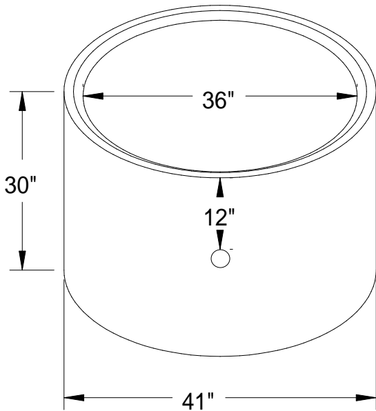
3 DIMENSIONAL VIEW OF WELL TILE
